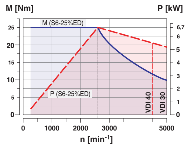
Tool turret motor characteristics for driven tools
