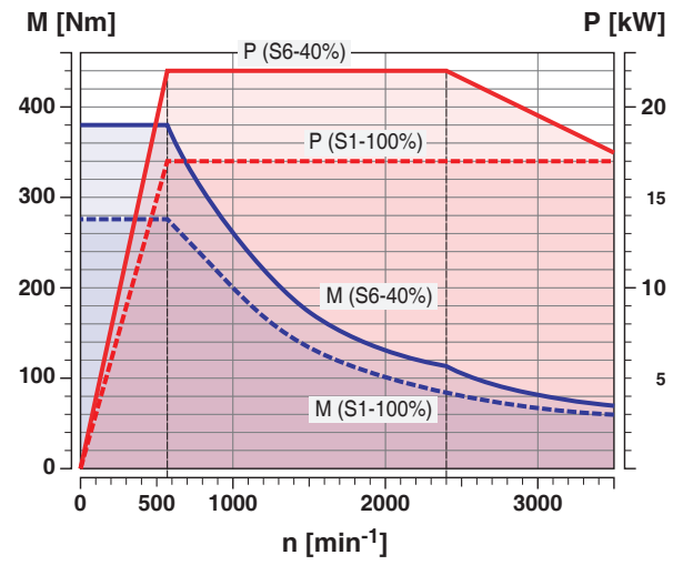
Motor characteristics for main spindle size 95
